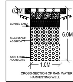
CROSS SECTION OF RAIN WATER HARVESTING WELL
